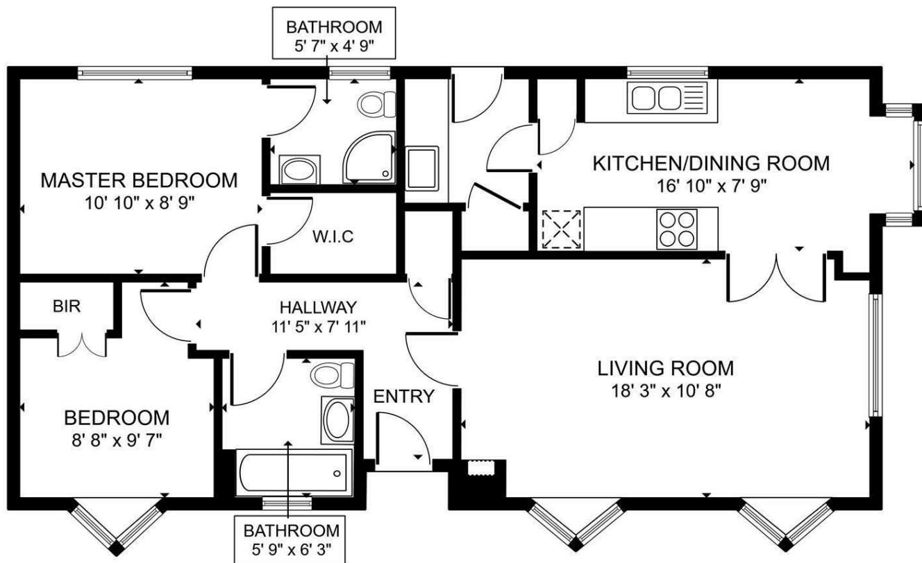
FLOOR PLAN
